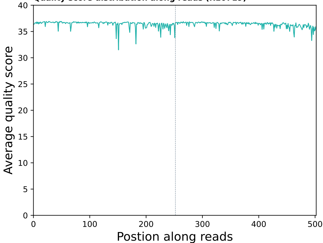
Quality score distribution along reads (R10719)
